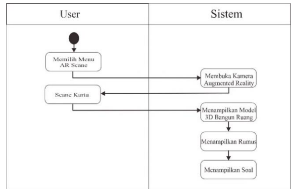
Gambar 4. Activity Diagram Menampilkan Objek 3D
